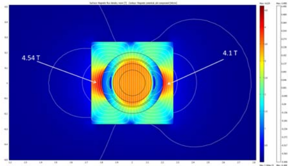
Figure 20. Saturated bent iron yoke.
