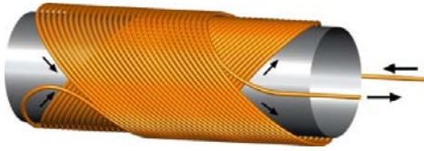
Figure 1. Example of a 2-layer winding used to form a DH dipole magnet
