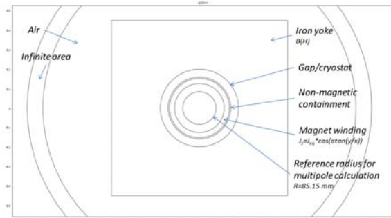
Figure 5. 2D model of a perfect dipole magnet
