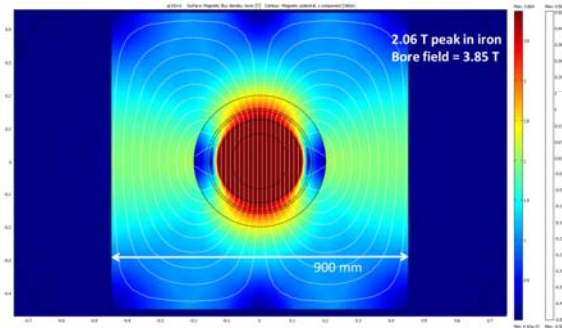
Figure 8. Perfect dipole magnet with iron yoke
