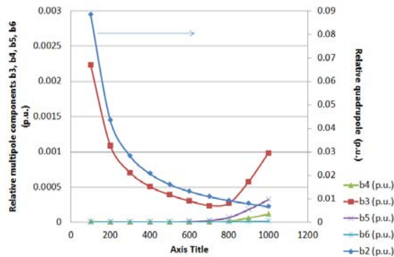
Figure 19. Magnitude of the multipole content of the bent magnet vs. excitation current
