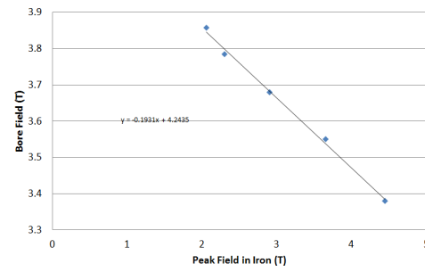
Figure 21. Bore field vs. peak field in the iron yoke
