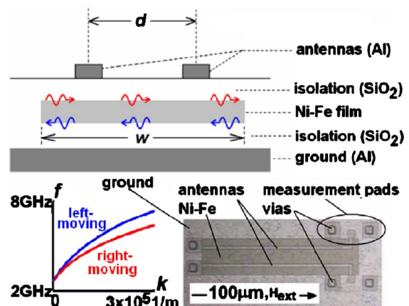
FIG. 1. (Color online) (Top) Schematic cross section of the coupled microstrip structure; two aluminum lines are coupled via surface waves propagating on a Ni–Fe layer. (Bottom left) Due to the presence of a metal ground close to the 200 nm thick Ni–Fe film, surface waves propagating in different directions have different dispersion characteristics, leading to nonreciprocal behavior. The nonreciprocity is enhanced by reducing the 1 \mu\text{m} ground-to-ferromagnet separation. (Bottom right) Top view microphotograph of a sample device, where the aluminum ground (background), rectangular patterned Ni–Fe core, microstrips acting as antennas, measurement pads, and via connections to the ground can be seen.
